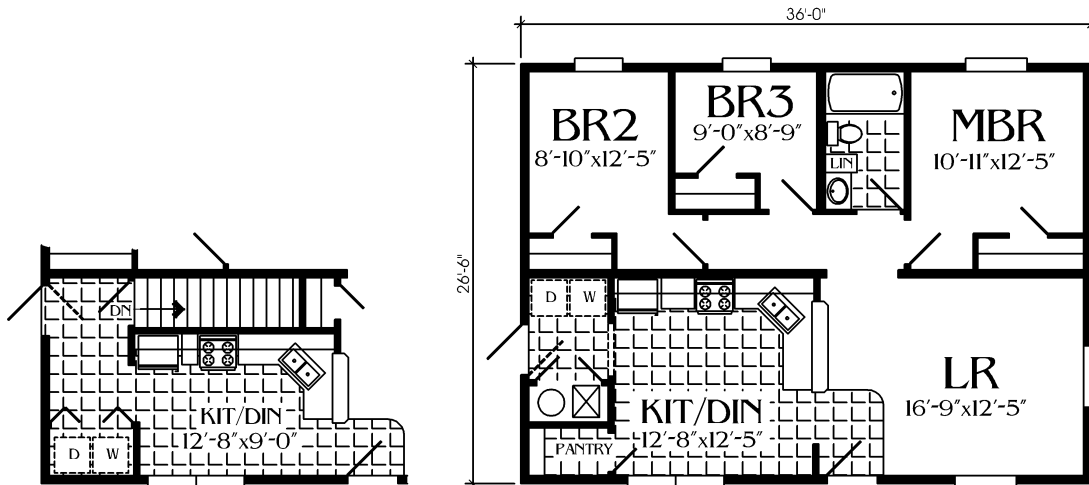
954 SQ. FT. Some room dimensions for HUD homes may be slightly larger than shown due to wall thicknesses.
