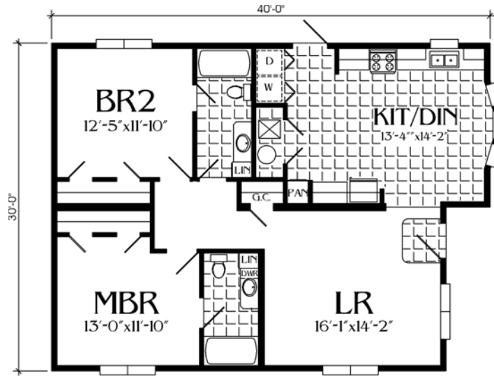
1140 SQ. FT. 2B, 2BA 324404 Some room dimensions for HUD homes may be slightly larger than shown due to wall thicknesses. MOD SERIES MODEL M4R40-K07 The Highland
