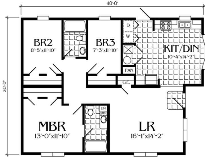
1140 SQ. FT. 3B, 2BA 324403 Some room dimensions for HUD homes may be slightly larger than shown due to wall thicknesses. MOD SERIES MODEL M4R40-K06 The Manhattan
