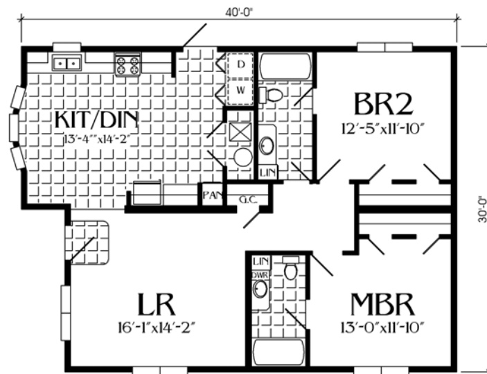
1140 SQ. FT. 2B, 2BA 324404E Some room dimensions for HUD homes may be slightly larger than shown due to wall thicknesses. MOD SERIES MODEL M4R40-K07E The Hopewell
