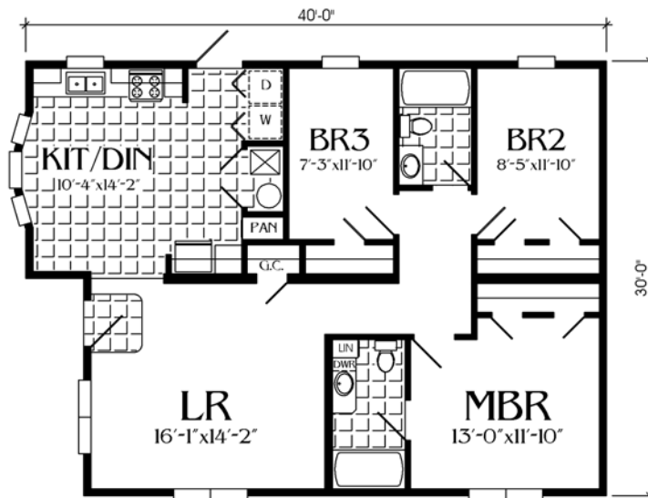
1140 SQ. FT. 3B, 2BA 324403E Some room dimensions for HUD homes may be slightly larger than shown due to wall thicknesses. MOD SERIES MODEL M4R40-K06E The Maywood
