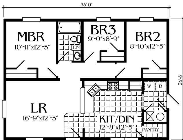
954 SQ. FT. Some room dimensions for HUD homes may be slightly larger than shown due to wall thicknesses.
